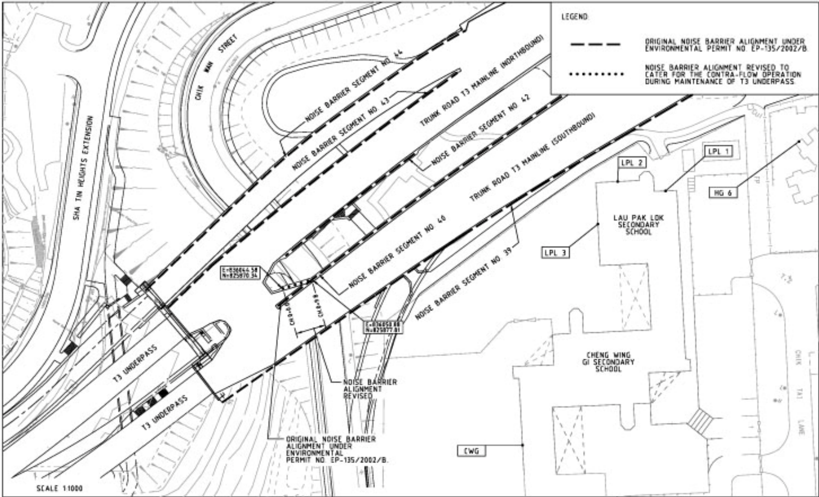
Figure 7 - Alignment of noise barrier segment no. 40 revised to cater for the contra-flow operation during maintenance of T3 Underpass.
